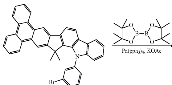
Intermediate II
