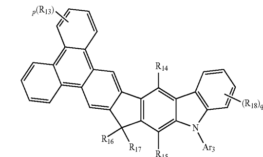
formula(I-2)
