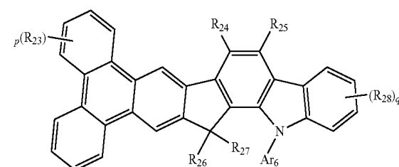
formula(I-4)
