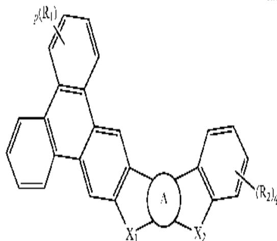
formula(I)
