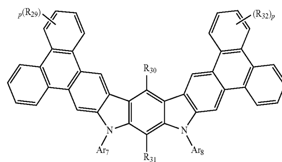
formula(II-2)
