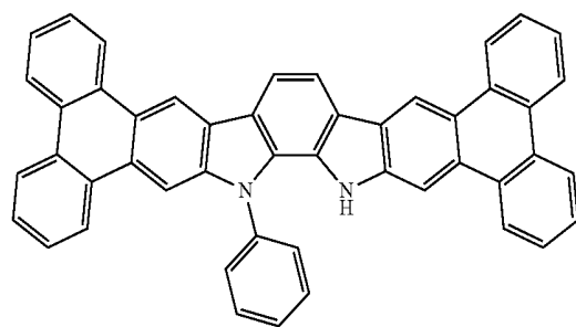
Intermediate C
