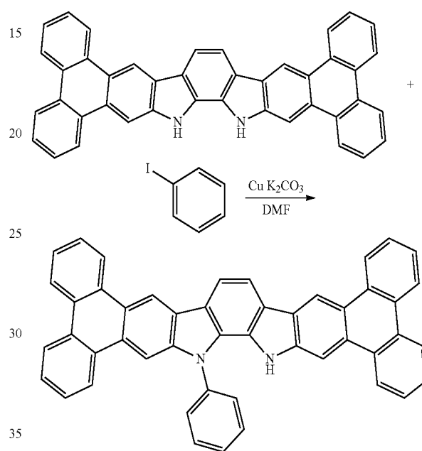
Intermediate C
