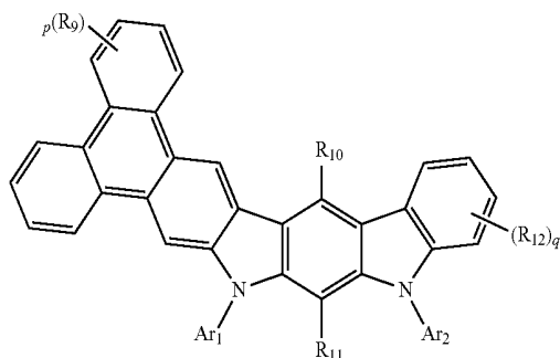
formula(I-1)
